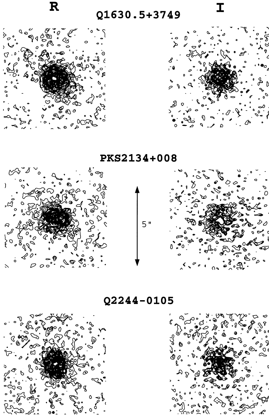
Figure 2. R - and I -band contour plots of the solutions found after performing a PSF subtraction that yields zero flux in the centroid of the QSO. The minimum contour level was set at 1\sigma of the sky noise after subtraction of the PSF. Further levels indicate 1\sigma increments over the minimum level. North is to the left, and east is down.
