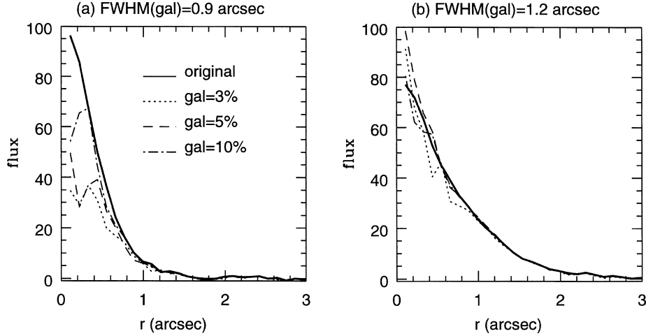
Figure 3. Results of flat-top PSF subtractions on simulated QSOs that use galaxies of (a) FWHM = 0.9 and (b) FWHM = 1.2 arcsec, with nuclear profiles of FWHM = 0.8 arcsec. The solid lines represent the original profiles of the galaxies before superposing the unresolved components. The dashed lines represent the recovered profiles of the galaxies after PSF subtraction. For the simulations presented here, the galaxies comprised 3, 5 and 10 per cent of the total luminosity of the simulated QSOs.
