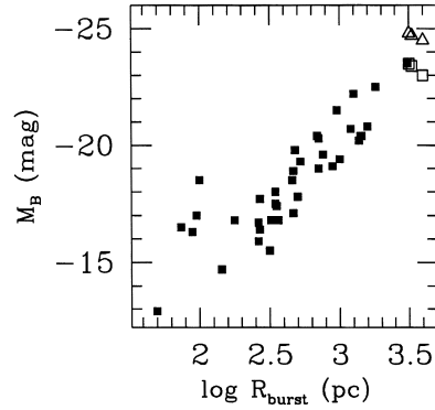
Figure 7. Luminosity–size relationship for nearby H\text{II} galaxies and QSO hosts. H\text{II} galaxies are marked with filled squares. The three QSOs studied here lie in this relation if their SEDs are f_\nu \propto \nu^0 (open triangles) to f_\nu \propto \nu^{0.5} (open squares). These SEDs are typical of young H\text{II} galaxies.
