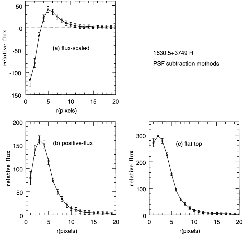
Figure 1. Radial profiles of the solutions found by performing PSF subtractions on the R -band frames of 1630.5+3749. Error bars represent the scatter around the mean value, and do not include the subtraction error. (a) flux-scaled subtraction; (b) subtraction to obtain zero flux at the position of the QSO centroid; (c) subtraction to obtain a smooth flat-top profile.
