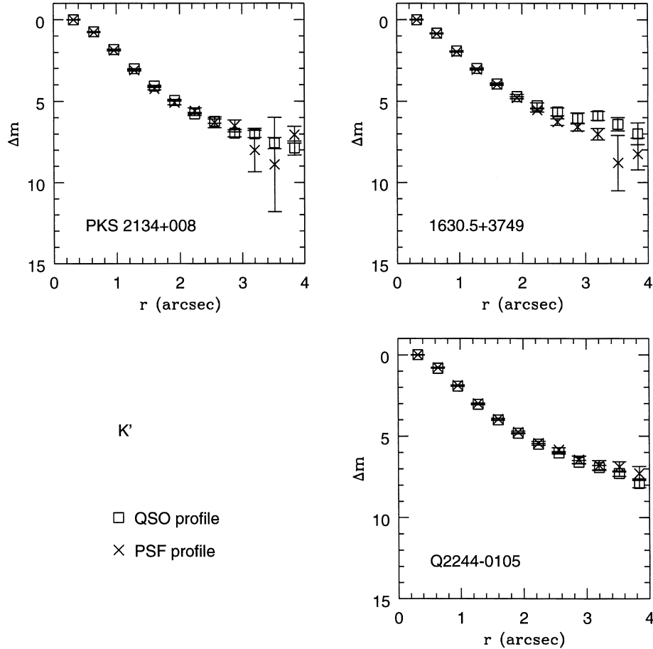
Figure 5. K' -band radial profiles of QSOs and stars in the field, normalized to their central flux.
