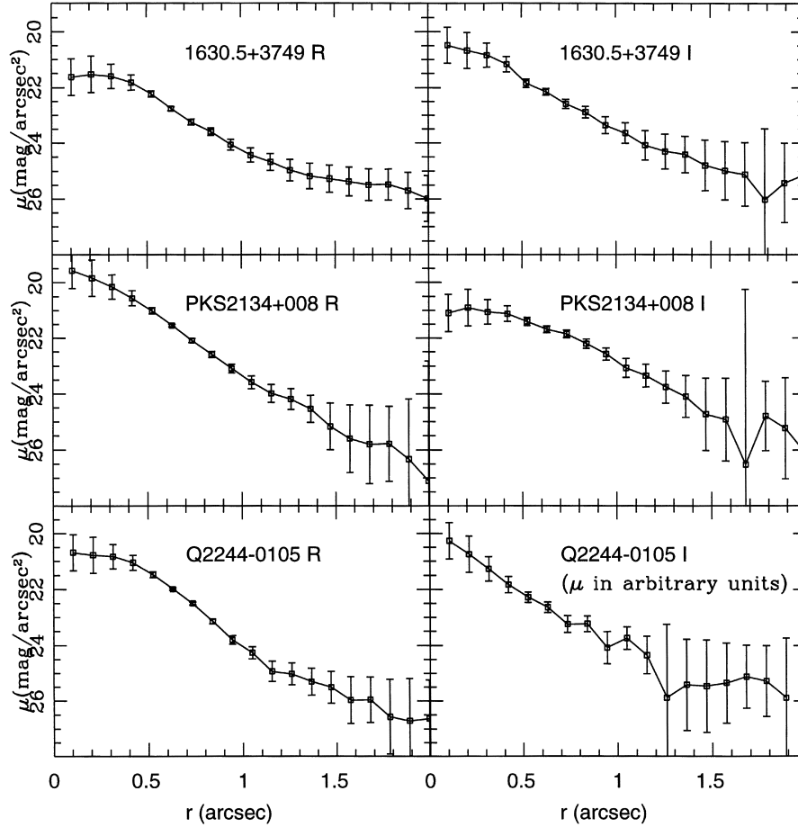
Figure 4. Radial profiles of the hosts derived from flat-top PSF subtractions. The error bars in the inner regions are dominated by the error in the subtractions, estimated from the simulations, and those in the outer regions are dominated by sky subtraction. The I -band profile of Q2244–0105 is not flux-calibrated.
