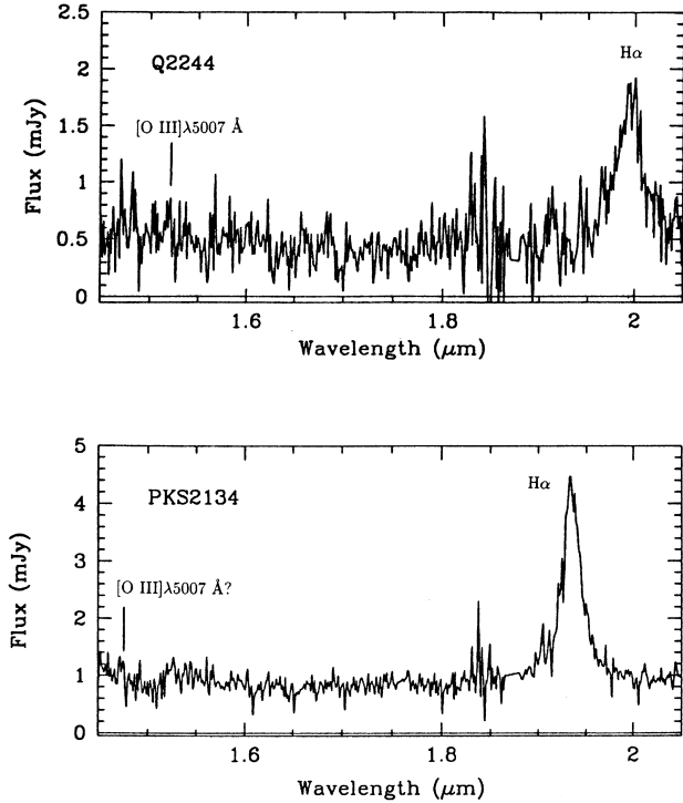
Figure 6. Near-IR spectra of the QSOs Q2244–0105 and PKS 2134+008.
