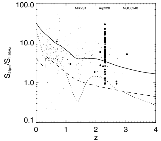
Figure 7. Ratio of S_{24\mu\text{m}}/S_{1.4\text{GHz}} as a function of redshift, z , for SHADES sources with robust counterparts (filled circles: LH; empty circles: SXDF). Those without spectroscopic redshifts – the majority – are plotted arbitrarily at z = 2.3 . The tracks of Arp 220, Mrk 231 and NGC 6240 are shown together with a sample of faint radio sources in SXDF (small dots – Ibar et al., in preparation).
