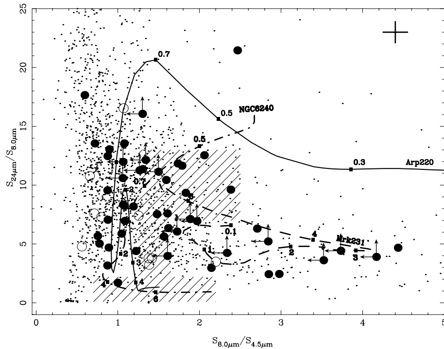
Figure 9. S_{24\mu\text{m}}/S_{8\mu\text{m}} versus S_{8\mu\text{m}}/S_{4.5\mu\text{m}} colour–colour diagram for a faint 24- \mu\text{m} -selected sample of 4457 galaxies (dots) with 4.5- and 8.0- \mu\text{m} detections. Robustly identified SMGs are plotted as filled circles and less securely identified SMGs as open circles. A representative error bar is shown, top right-hand side. The redshift tracks of Arp 220, Mrk 231 and NGC 6240 are shown (adopting SEDs from Rigopoulou et al. 1999 and Spoon et al. 2004), with squares to indicate redshift. Hatched regions indicate regions of colour–colour space where one might expect to find the most distant SMGs.
