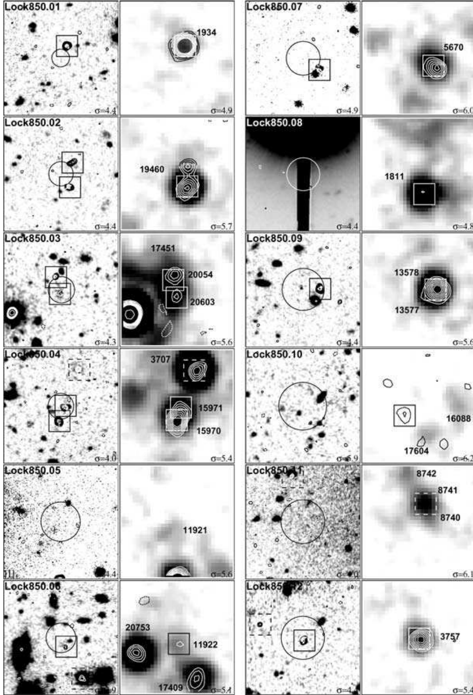
Figure A1. 25 × 25-arcsec postage stamp images of each SMG in the LH SHADES Source Catalogue. Grey-scale R -band and 24- \mu m data are shown in the left- and right-hand panels, respectively, superimposed with radio contours. Circles indicate 2\sigma positional uncertainties. Solid boxes indicate robust identifications, where P \leq 0.05 based on the radio or 24- \mu m counts, or a combination of the two. Dashed boxes indicate tentative associations.
