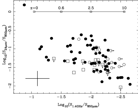
Figure 8. \log_{10} S_{24\mu\text{m}}/S_{850\mu\text{m}} versus \log_{10} S_{1.4\text{GHz}}/S_{850\mu\text{m}} for SHADES SMGs with both mid-IR and radio identifications (filled circles), with only radio identifications (squares) and with only mid-IR identifications (open circles). A representative error bar is shown, lower left-hand side. The redshift parametrization of Chapman et al. (2005) is shown as a horizontal bar at \log_{10} S_{24\mu\text{m}}/S_{850\mu\text{m}} = 0 (see Section 7.2).
