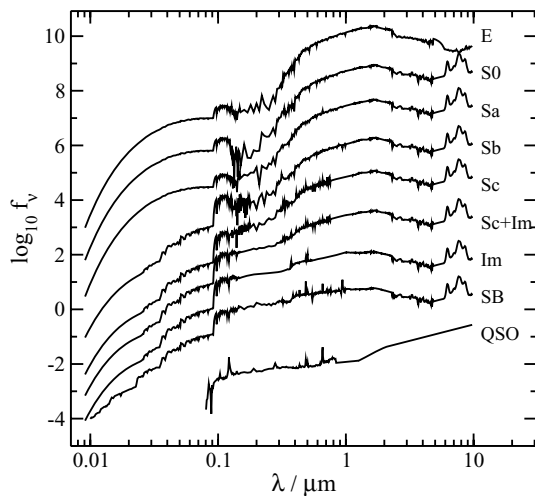
Figure 1. Template SEDs used with HYPERZ for determination of the photometric redshifts. The template Sc + Im is a hybrid SED composed of 60 per cent Sc and 40 per cent Im to bridge the jump between the Sc and Im types (see text). SED templates are referred to throughout this paper by their number: 1 = E, 2 = S0, 3 = Sa, 4 = Sb, 5 = Sc, 6 = Sc + Im, 7 = Im, 8 = starburst, 9 = QSO.
