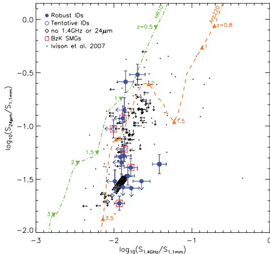
Figure 4. S_{24\mu\text{m}}/S_{1.1\text{mm}} versus S_{1.4\text{GHz}}/S_{1.1\text{mm}} for SMGs in the MS0451–03 field. We differentiate between sources with robust and tentative detections ( 0.05 < P \leq 0.10 ), and highlight SMGs which satisfy the BzK selection criteria of Daddi et al. (2004) (Fig. 5). Sources without both mid-IR and radio detections are plotted at the 3\sigma detection limit of the respective catalogues (Table 1). For comparison we also plot SHADES identifications (Ivison et al. 2007), converted to expected observed 1.1 mm fluxes as discussed in the text; error bars of this sample are omitted for clarity. Both sets of SMGs lie broadly within the same region of colour–colour space, providing confidence in our identifications. Redshift tracks of the z = 1.4 SMG HR10 and local starburst Arp 220 [based on SEDs from Silva et al. (1998)] suggest that the AzTEC sources generally have 1 \lesssim z \lesssim 3.5 , in concordance with Chapman et al. (2005).
