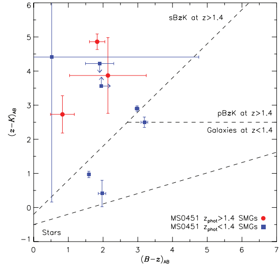
Figure 5. B - z versus z - K colour–colour plot of the optically identified AzTEC galaxies in MS0451–03 which lie within the field-of-view of our B , z and K observations. The lines of separation between passive and star-forming z > 1.4 BzK galaxies (pBzK and sBzK, respectively), z < 1.4 galaxies and stars (Daddi et al. 2004) are shown. Two SMGs occupy the z < 1.4 region, suggesting they are potential cluster members. We distinguish between galaxies with z_{\text{phot}} > 1.4 and z_{\text{phot}} < 1.4 based on photometric redshifts calculated in Section 3.3.3. The BzK selection and full photometric analysis broadly agree as to the high- and low-redshift samples giving more confidence in our ability to isolate millimetre sources in the cluster from the dominant background population. As expected, by these criteria most SMGs are deemed to be actively star forming.
