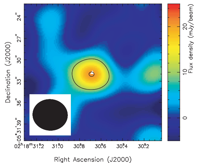
Figure 8. The SMA 880- \mu\text{m} image of the extended component of Orochi, produced by the residual visibility data after subtracting unresolved component in the uv domain (See Section 5.1). The contour levels are 2.5\sigma and 5\sigma ( 1\sigma = 4.1 mJy). The synthesized beam is shown on the lower left. The white triangle marks the position of the compact component.
