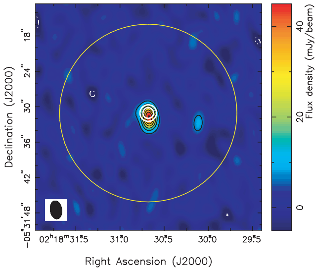
Figure 3. The SMA 880- \mu\text{m} image of Orochi. The contour levels are -3\sigma , 3\sigma , 6\sigma , 9\sigma , 12\sigma , 15\sigma , 18\sigma and 21\sigma ( 1\sigma = 2.2 \text{ mJy} ). Negatives are shown in white contours. The synthesized beam is shown on the lower left. Note that no correction of the primary beam attenuation was made in this map. The large solid yellow circle shows the beam size of AzTEC/ASTE (30 arcsec). The small solid white circles show the estimated position errors; the inner one shows 1\sigma error (0.9 arcsec) and the outer one shows 2\sigma error (1.4 arcsec).
