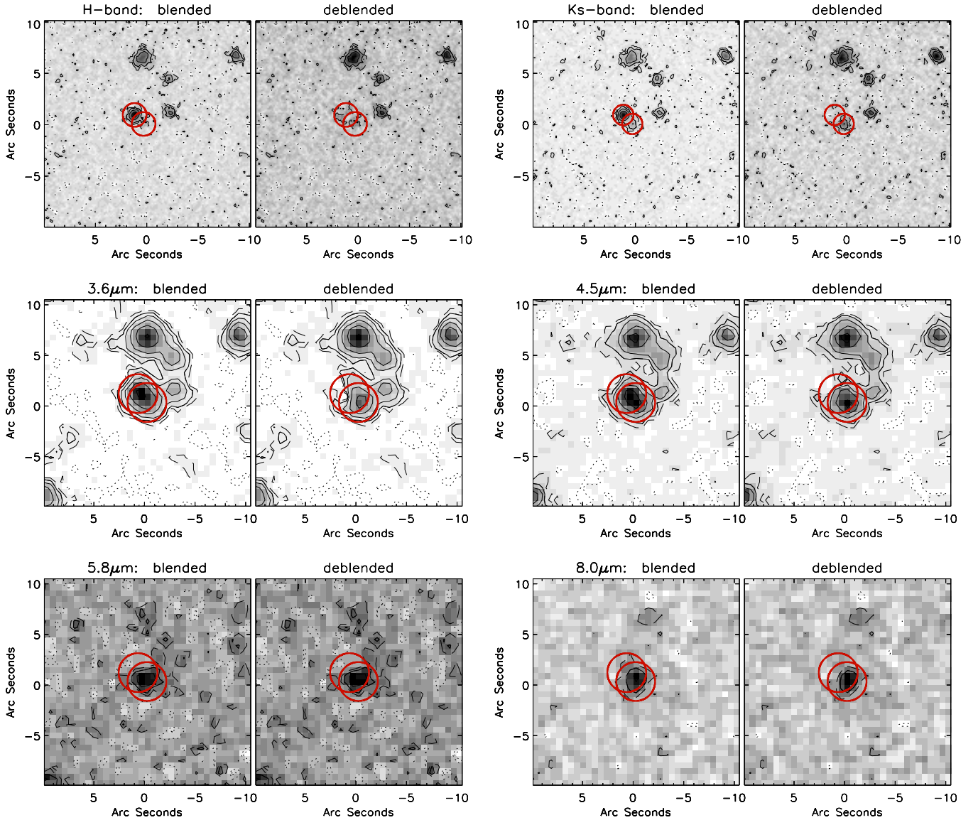
Figure 4. Blended and deblended Cosbo-8 images. H , Ks , and IRAC bands (indicated in each panel) needed to be deblended. The contour levels are at -4\sigma , -2\sigma (dotted lines), 2\sigma , 4\sigma (dashed lines), and 2^i\sigma , i = 3, 4, 5, 6, \dots (full lines), where the rms ( \sigma ) has been derived locally. The CARMA position is marked by the thick circle in the center of the stamp (its size matches the photometry aperture). The source that was subtracted (assuming a 2D Gaussian point-source model) is outlined by the circle to the NE.
