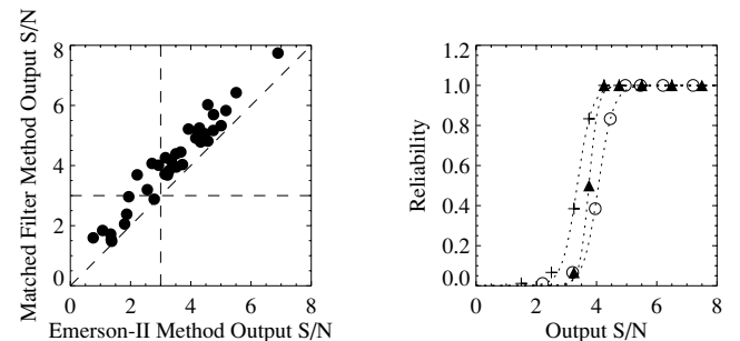
Figure 6. Left: comparison of the output S/N of the input sources for the matched-filter and Emerson-II deconvolution methods, for the simulations shown in Fig. 5. The dashed lines show \text{S/N} = 3 for each of the methods, and the line for which the two methods would have equal S/N. Right: the reliability of sources extracted from the matched-filter method (filled triangles) and Emerson-II deconvolved maps (crosses). This is based only on the sources in the top-left-hand panel, which is far fewer than the more extensive simulations in Fig. 8; however, since these are the same sources being extracted in both matched-filter and Emerson-II methods, the relative reliabilities can still be usefully compared. For a fixed S/N, the reliability appears to be higher for the raw Emerson-II deconvolution, but this is easily shown to be an artefact of the poorer S/N of Emerson-II for a fixed input flux (left). After adjusting for the poorer S/N in the Emerson-II method (open circles), the reliability is shown to be less for the Emerson-II deconvolved maps than the matched-filter method. Thus, for example, a 3.5\sigma source in an Emerson-II map is intrinsically brighter than a 3.5\sigma source in a matched-filter map, and it is unremarkable that such brighter sources can be extracted more reliably; however, an 8-mJy source extracted from an Emerson-II map has a lower reliability than an 8-mJy source from a matched-filter extraction.
