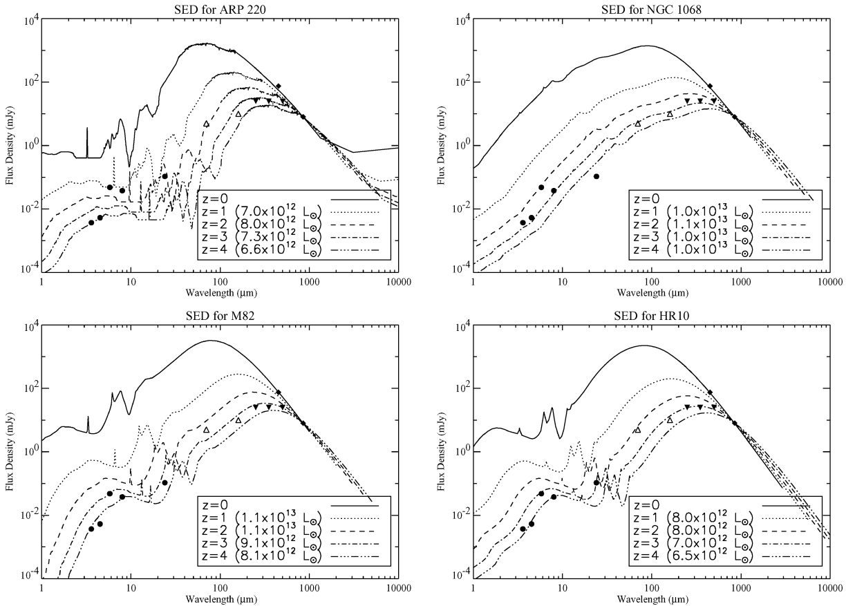
Figure 1. Model spectral energy distribution (SED) plots of template galaxies with survey sensitivities overplotted. Filled circles: SWIRE sensitivities 500 s, 5 \sigma (Lonsdale et al. 2004). Open triangles: the pre-flight Spitzer sensitivities for 70 and 160 \mu\text{m} are shown whilst the SWIRE team reassesses its observing strategy due to the degraded MIPS sensitivities, although currently these are expected to be two to three times worse. Filled triangles: the pre-flight BLAST confusion limit estimates [derived from Rowan-Robinson (2001)] of 25 mJy; the sensitivity estimates (Hughes et al. 2002) are in the range 15–25 mJy. Filled diamonds: SHADES survey sensitivities of 8 mJy at 850 \mu\text{m} and 75 mJy at 450 \mu\text{m} . Models have been normalized to the SHADES survey depth of 8 mJy at 850 \mu\text{m} . Top left-hand panel: Arp 220 – a highly obscured local starburst galaxy [note: it is also a ULIRG Elbaz et al. (2002)]. Top right-hand panel: NGC1068 – a typical Seyfert galaxy (Efstathiou, Hough & Young 1995). Bottom left-hand panel: M82 – an irregular dusty star-forming galaxy (Efstathiou et al. 2000). Bottom right-hand panel: HR10 – a high-redshift and extremely-red galaxy (Takagi, Hanami & Arimoto 2004). Bolometric (3–1000 \mu\text{m} rest frame) luminosities for each model, as normalized, are shown in the legends.
