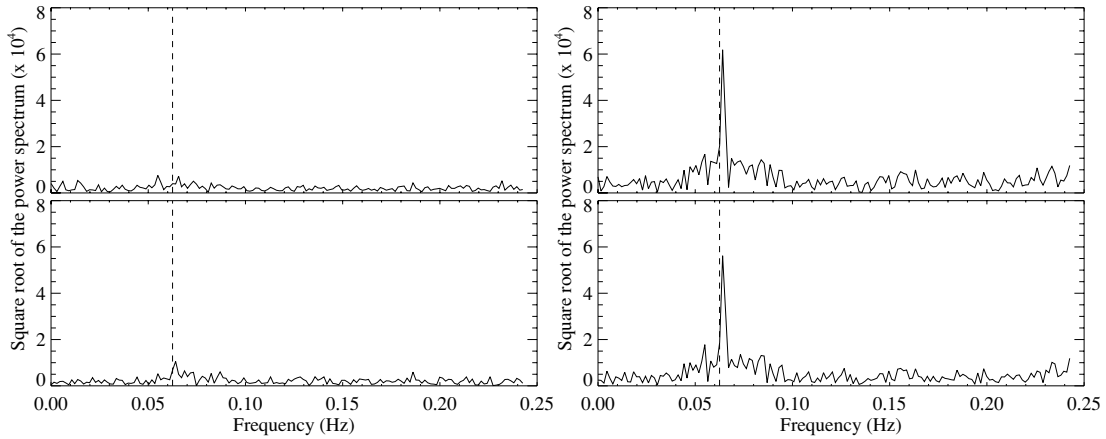
Figure 3. The spike in the power spectrum of the bolometer readouts. The left-hand column of plots shows the power spectrum of a typical (in this case the central) bolometer, before (top) and after (bottom) sky subtraction. The right-hand column of plots shows the same for a bolometer affected by the power spike, showing clearly the spike at a period of roughly 16 samples (at the dotted line) and the fact that the power spike itself has not changed.
