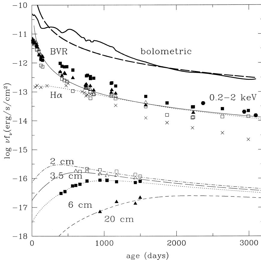
Figure 2. Evolution of the \nu f_\nu light curve in radio to X-ray bands. In the upper part of the panel, open triangles correspond to the B -band, solid triangles to the V -band, solid squares to the R -band, empty squares to R_{\text{cont}} band, solid hexagons to the ROSAT 0.2–2 keV band and crosses to H\alpha . The thin solid and dashed lines are models for the bolometric light (scaled to the values of the optical data) and H\alpha evolution of a cSNR. In the lower part of the panel, the VLA radio data at 2, 5.5, 6 and 20 cm is represented with empty squares, empty triangles, solid squares and empty triangles. The line fittings correspond to the models of Van Dyk et al. (1993). The thick solid line at the top of the panel shows the strong lower limit estimate, while the thick dashed line represents our best estimate of the bolometric light curve of SN 1988Z (see Section 4.2).
