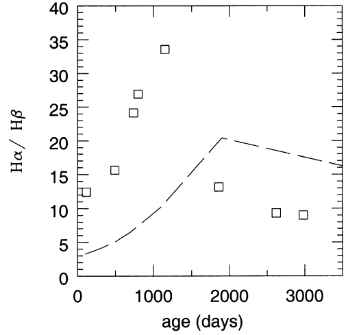
Figure 8. Evolution of the Balmer decrement (empty squares). The dashed line represents the theoretical values for the evolution of a cSNR
