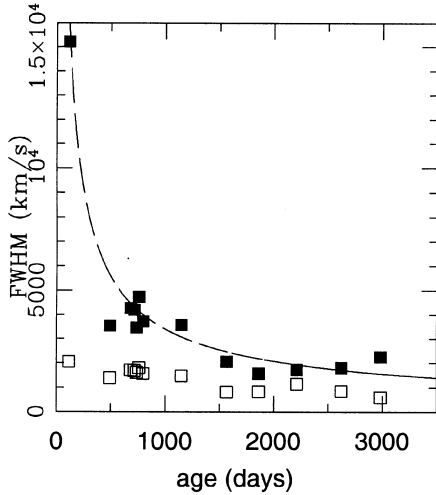
Figure 7. Evolution of the H\alpha line profile. Solid squares represent the broad component and empty squares represent the intermediate component. The dashed line represents the law for the velocity shock evolution of a cSNR.
