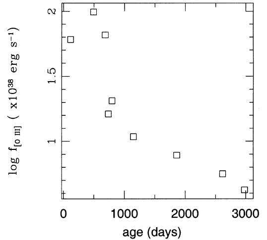
Figure 9. Evolution of [O\text{ III}]\lambda 5007 line.
