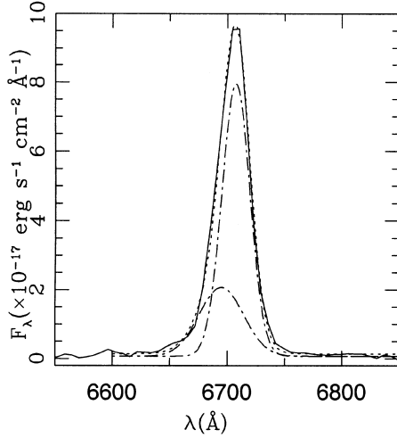
Figure 6. Multicomponent fit of the H\alpha line of the spectrum taken on 1996 February 14. The parameters of the components are given in Table 5. The dot-dashed lines represent single Gaussian components, while the solid line and dotted line represent the spectrum and the fit.
