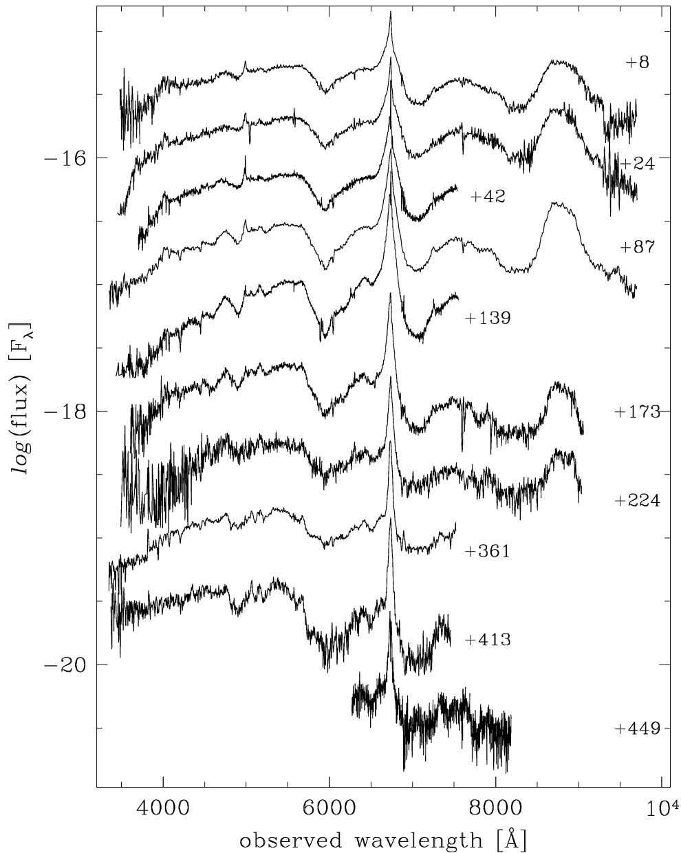
Figure 3. Spectral evolution of SN 1999E. The ordinate refers to the first spectrum, and the others have been arbitrarily shifted. The phase (days) is from the discovery date (1999 January 15). The spectra shown have been obtained with the following instruments: phase +8 d, Danish 1.5-m telescope at La Silla + DFOSC, resolution 12 \text{ \AA} ; +24 d, ESO 1.5 + B&C, res. 15 \text{ \AA} ; +42 d, William Herschel telescope at La Palma +ISIS, res. 3.1 \text{ \AA} ; +87 d, ESO 3.6 m + EFOSC2, res. 17 \text{ \AA} ; +139 d, ISIS, res. 3.1 \text{ \AA} ; +173 d, DFOSC, res. 12 \text{ \AA} ; +224 d, DFOSC, res. 12 \text{ \AA} ; +361 d, EFOSC2, res. 18 \text{ \AA} ; +413 d, EFOSC2, res. 18 \text{ \AA} ; +449 d, EFOSC2, res. 6.5 \text{ \AA} .
