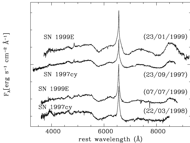
Figure 4. Comparison of the spectra of SN 1999E and SN 1997cy, corrected to the parent galaxy rest frames. The two spectra at the top have been obtained approximately 135 d past the GRB to which the SNe are possibly associated (+8 d past discovery for SN 1999E); those at the bottom approximately 300 d (+173 past discovery for SN 1999E). The ordinate scale refers to the top spectrum of SN 1999E, other spectra have been arbitrarily downshifted. The bottom two spectra have also been multiplied by a factor of 2 for an easier comparison.
