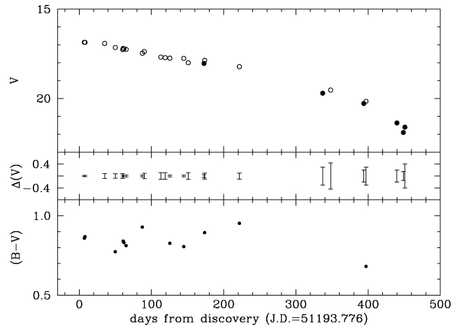
Figure 1. Top: V light curve of SN 1999E. Open symbols represent measurements performed with the PSF fitting technique and filled symbols represent those performed with the background subtraction method. Middle: estimates of the errors of the photometry performed via artificial star experiments. Bottom: ( B – V ) colour curve of SN 1999E.
