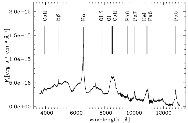
Figure 6. Line identifications in the optical-IR spectrum of SN 1999E (taken on 1999 March 11 with 1.5 m + B&C, phase +55 d, and 1999 March 7 with NTT+Sofi, phase +51 d) shifted to the rest frame of the host galaxy.
