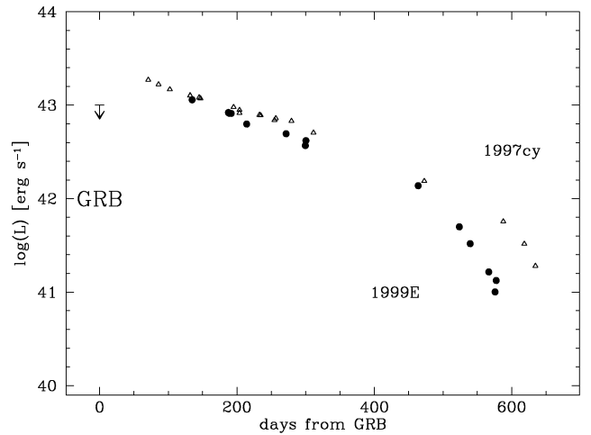
Figure 7. Comparison of the UBVR bolometric light curve of SN 1999E with that of SN 1997cy when the phase is computed from the respective GRB.
