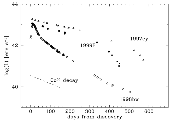
Figure 2. UBVRI bolometric light curve of SN 1999E compared with those of the hypernovae 1998bw (Patat et al. 2001) and 1997cy (Turatto et al. 2000). For each SN the luminosities are plotted versus the days from discovery. The last estimates have been scaled from the V magnitudes only. The dashed line corresponds to the ^{56}\text{Co} to ^{56}\text{Fe} decay rate, expected for full \gamma -ray trapping.
