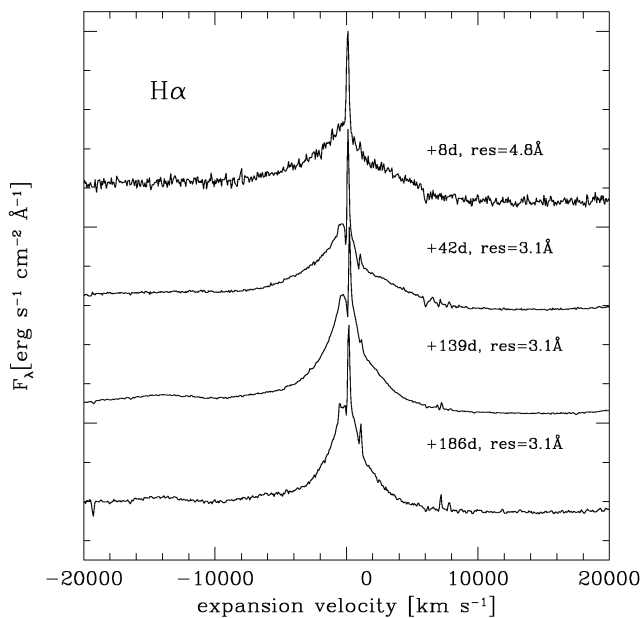
Figure 5. Time evolution of the H\alpha profile from the higher-resolution spectra. The line fluxes have been normalized to the peak intensities. Broad wings and narrow unresolved emissions and absorptions are visible.
