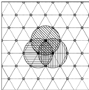
Figure 2. The ‘triplos’ positioning scheme. Individual jiggle-maps (2.6-arcmin diameter) are represented as large hatched circles; only three of these are plotted for clarity, but the centres of the others are marked with small open circles. This pattern of overlapping jiggle maps, in conjunction with observing different chop-throw/PA combinations at different airmasses, provides an approximately uniform coverage over the map. These three hatched jiggle maps, with centres marked by filled circles, comprise one ‘triplos’. Only these three positions contribute to the data within the triple-hatched triangle formed by the filled circles. Any other triangular region is covered by its own combination of three jiggle-maps. The jiggle-map positions shown by the open circles are observed sequentially in a spiral manner from the centre of the map outwards; the resulting roughly circular areal coverage minimizes the perimeter, which has lower coverage and so lower S/N than the rest of the survey.
