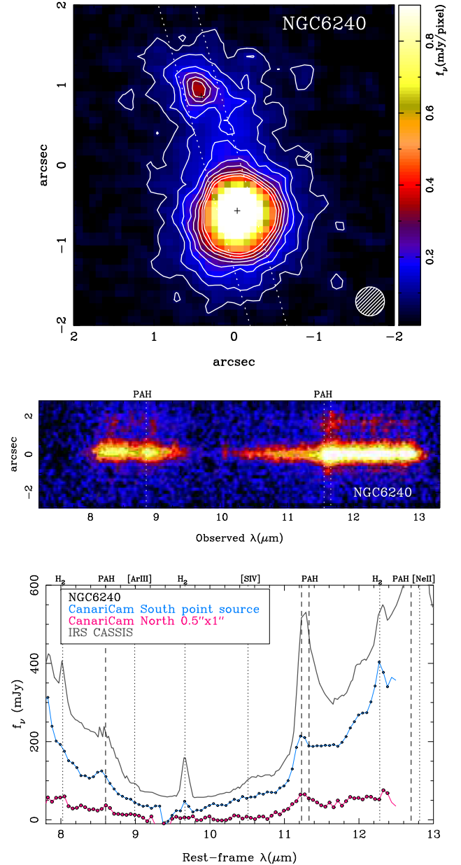
Figure 4. NGC 6240. Symbols as in Fig. 1. The top panel is the GTC/CanariCam 8.7\ \mu\text{m} image smoothed with a Gaussian function with \sigma = 0.7 pixels. The contours are in a linear scale with the lowest contour corresponding to the local background value plus 1.5 standard deviations measured in the image before rotating and smoothing the images. The crosses indicate the positions of the radio sources (Beswick et al. 2001) after we made the radio southern source coincident with the bright mid-IR southern nucleus. The middle panel is the partially reduced GTC/CanariCam 2D spectrum. On the y-axis positive offsets indicate north-east and negative offsets south-west. The northern nucleus is located at approximately +1.5 arcsec from the southern nucleus. In the bottom panel are the 1D GTC/CanariCam spectra (smoothed as in Fig. 1, bottom panel) through extraction apertures centred on the southern and northern nuclei compared to the Spitzer /IRS SL spectrum, which encompasses both nuclei.
