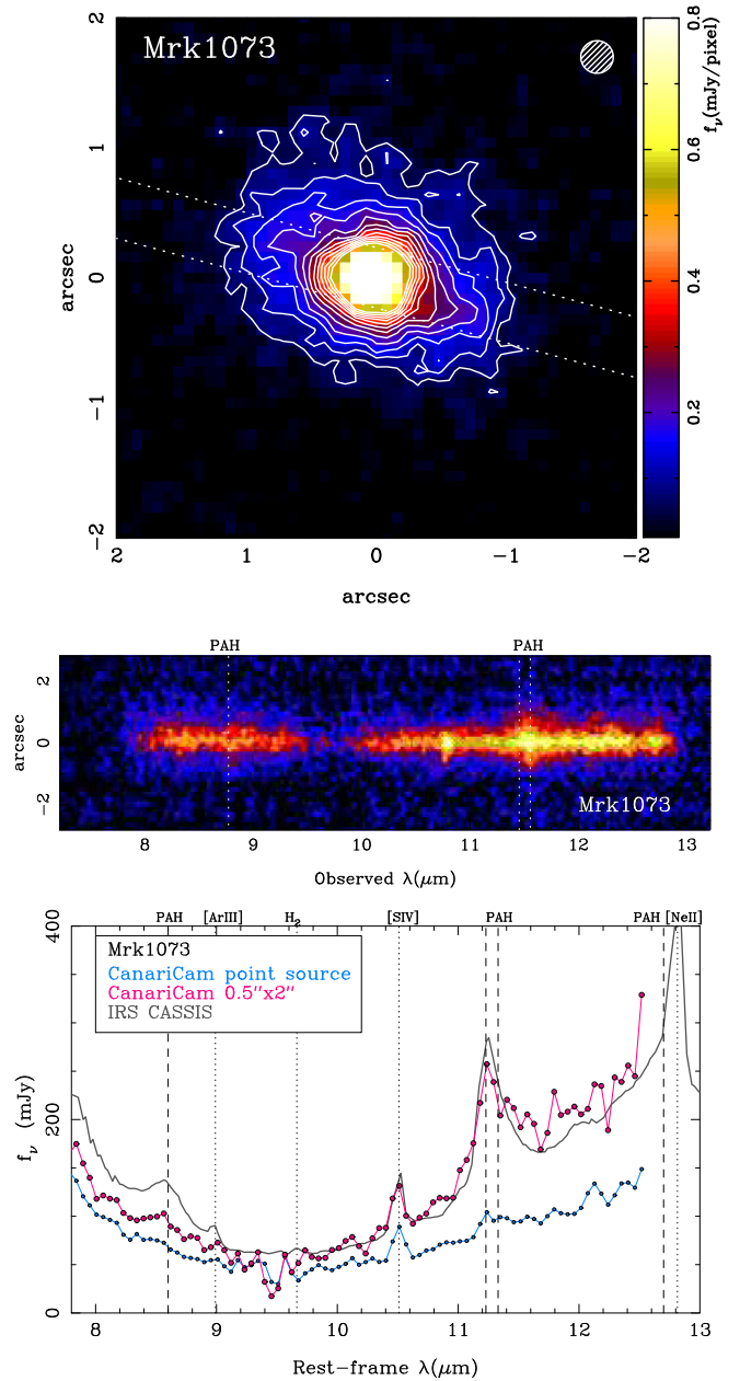
Figure 2. Mrk 1073. Symbols as in Fig. 1. The top panel is the GTC/CanariCam 8.7 \mu\text{m} image smoothed with a Gaussian function with \sigma = 0.6 pixels. The contours are in a linear scale with the lowest contour corresponding to the local background value plus two standard deviations measured in the image before rotating and smoothing the images. The middle panel is the partially reduced GTC/CanariCam 2D spectrum. On the y-axis positive offsets indicate north-east and negative offsets south-west. The bottom panel compares the 1D GTC/CanariCam spectra (smoothed as in Fig. 1, bottom panel) and the Spitzer /IRS spectrum. The GTC/CanariCam 0.52 \text{ arcsec} \times 2 \text{ arcsec} spectrum of Mrk 1073 was scaled down by a factor of 1.8 to match the IRS one.
