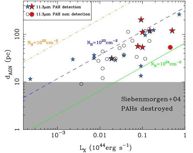
Figure 13. Diagram showing regions of PAH survival as a function of the distance from the AGN and the AGN X-ray luminosity according to the modelling of Voit (1992) and Miles et al. (1994). The lines of constant total column densities [lines from top to bottom N_{\text{H}}(\text{tot}) = 10^{22}, 10^{23}, 10^{24} \text{ cm}^{-2} ] of the intervening material define the regions above which PAHs would be protected and not destroyed by the AGN radiation field. The shaded area shows the region where PAHs would not survive ( d_{\text{AGN}} \leq 10 \text{ pc} ) according to the modelling of Siebenmorgen et al. (2004). Galaxies with a nuclear detection of the 11.3 \mu\text{m} PAH feature are shown as small and large star-like symbols for RSA galaxies from Esquej et al. (2014) and this work, respectively. Circles are galaxies with non-detections of the nuclear PAH feature. For the galaxies, the plotted X-ray luminosities are intrinsic (corrected for absorption) 2–10 keV luminosities and d_{\text{AGN}} are projected distances.
