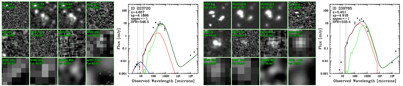
Figure 30. Multiband cutouts and SEDs of high-redshift candidates.
