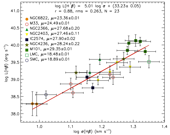
Figure 1. L(\text{H}\beta) - \sigma relation for the GEHR sample. The correlation parameters and the adopted individual distance moduli are given in the inset. The line is the best fit for the slope determined by the fit to the H II galaxies (see Eq. 3).
