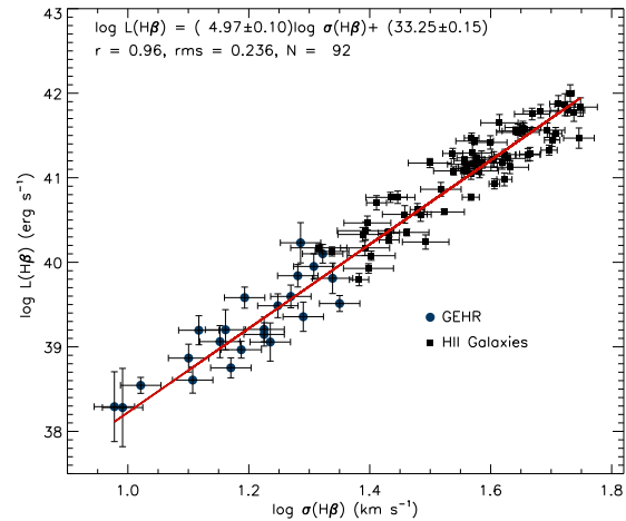
Figure 2. L(\text{H}\beta) - \sigma relation for the joint H II galaxies and GEHR samples. The least square fit considers the errors in both axes.
