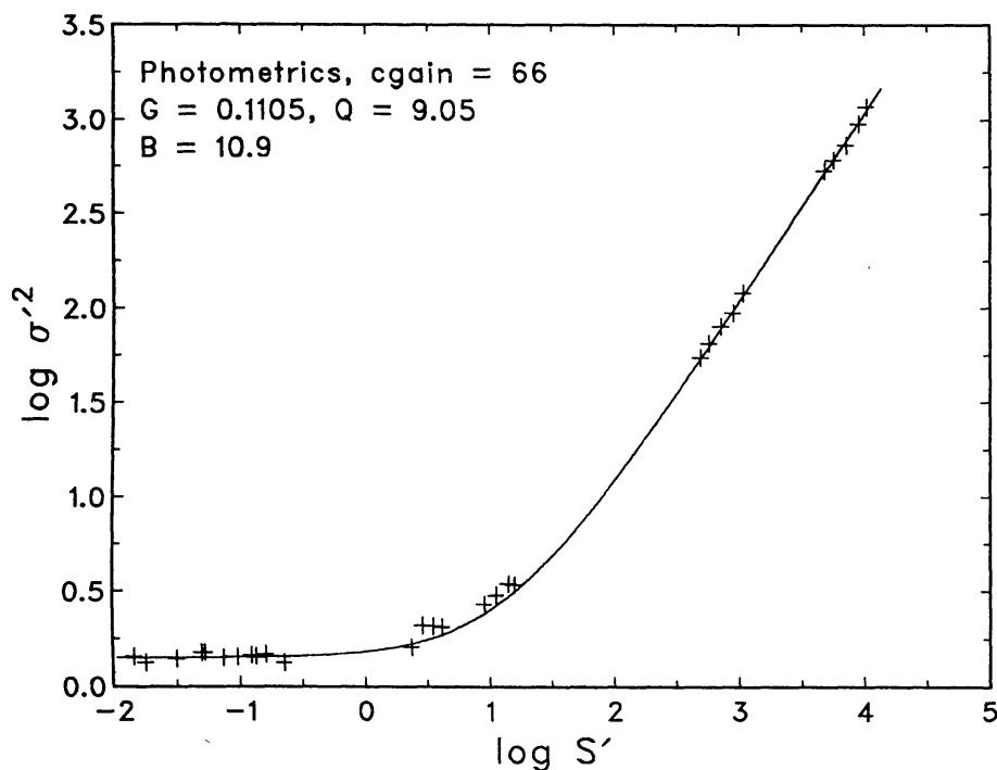
Figure 3. The logarithmic plot of variance versus signal together with the theoretical fit for the Photometrics CCD system and \text{cgain} = 66 . The fit is based on data in the range S > 500 , and the bias statistics. Other details are as in Fig. 1.
