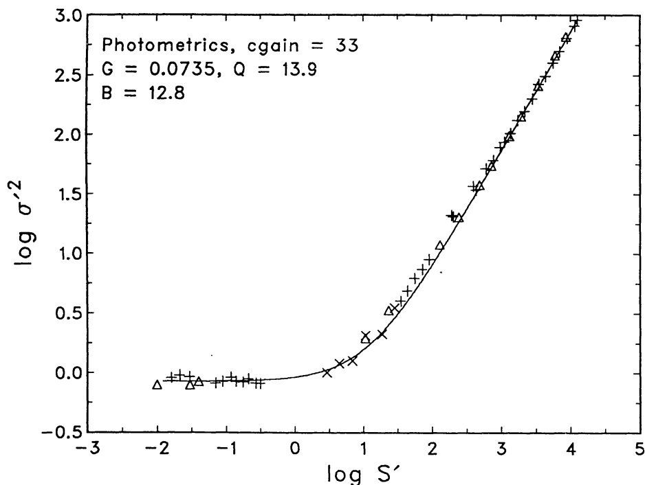
Figure 2. The logarithmic plot of variance versus signal together with the theoretical fit for the Photometrics CCD system and \text{cgain} = 33 based on the data obtained in 1992 January. The fit is based on spectroscopic data in the range 300 \leq S \leq 10000 , and the bias statistics. Other details are as in Fig. 1. Surprisingly, data from a different set ( \times ) obtained on 1991 May 12, agrees with the theoretical fit even at low signal values.
