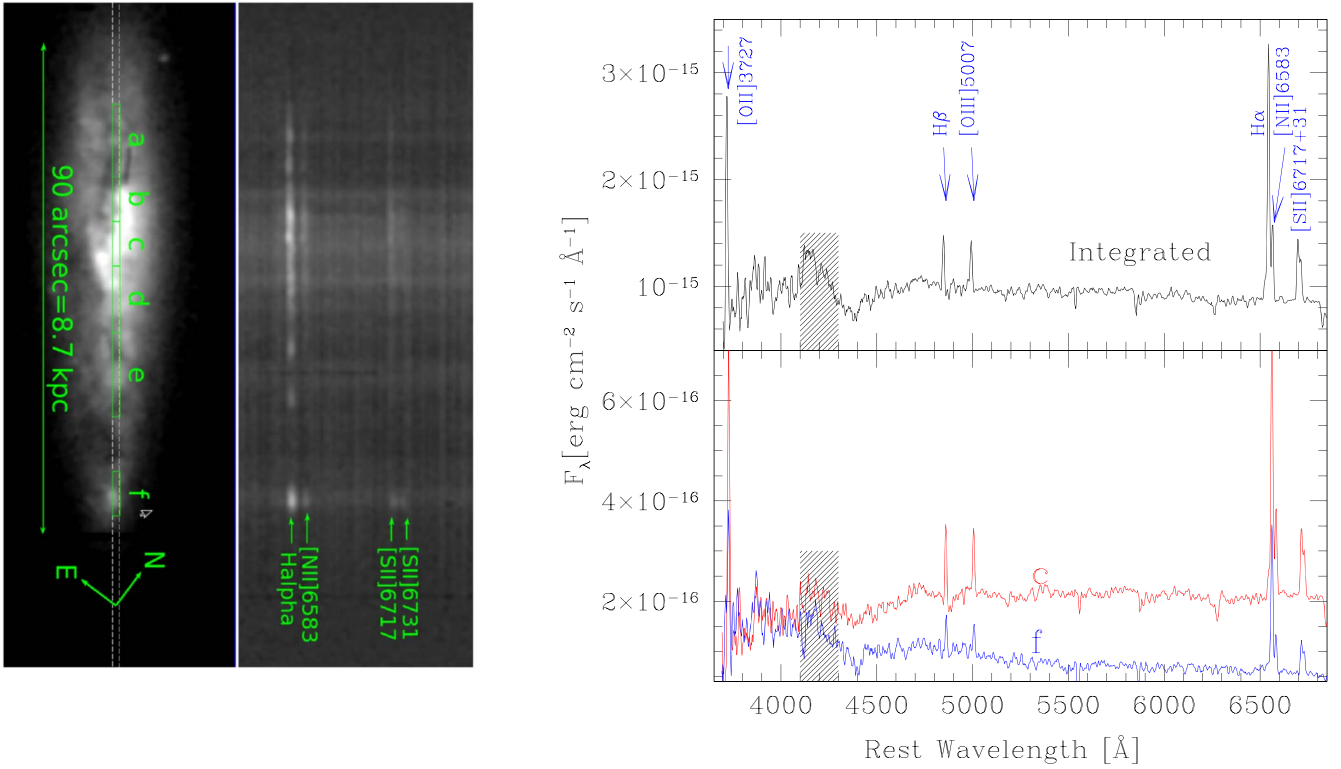
Figure 7. (Left) GTC/OSIRIS r -band acquisition image showing the position of the long slit (white dashed rectangle; PA = 37^\circ 31' ) and the zones a–f selected for the spectral extraction (green rectangles). The image scale and orientation are shown. (Center) Spectral image along the long slit showing prominent emission lines in the red part of the spectrum. (Right) Rest-frame spectra, where the top spectrum was obtained by summing the rest-frame spectra of all the six zones denoted a–f. Spectra marked “c” and “f” correspond to the zone passing through the nucleus and a bright H II, respectively. Note that the latter region lies almost at the center of the 90% localization ellipse of the FRB source shown (see Figure 2). A bump in the spectra between 4100 and 4300 Å is due to a detector artifact, which is shown by shaded box.
